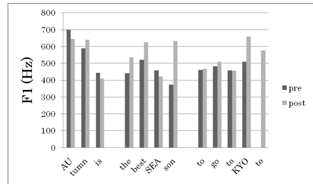
Fig. 5. F1 patterns of pre and post-training utterances for most improved student in Class 2.
