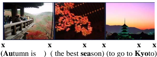
Fig. 1. Images are presented synchronously with metronome and verbal phrases; x's indicate timing of metronome beat—one on the stressed syllable of the phrase and another at the phrase break; the utterance is written with parentheses indicating the phrases associated with each image above.
