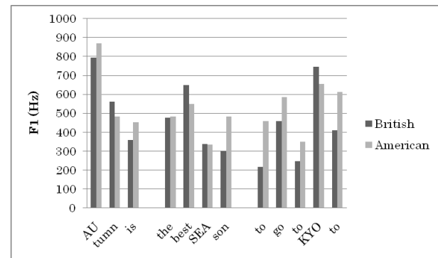
Fig. 2. F1 values for each syllable are shown for the British (dark) and American (light) teacher. The three phrases are indicated by breaks in the bargraph. The stressed syllables in each of the phrases is are indicated by capital letters.
